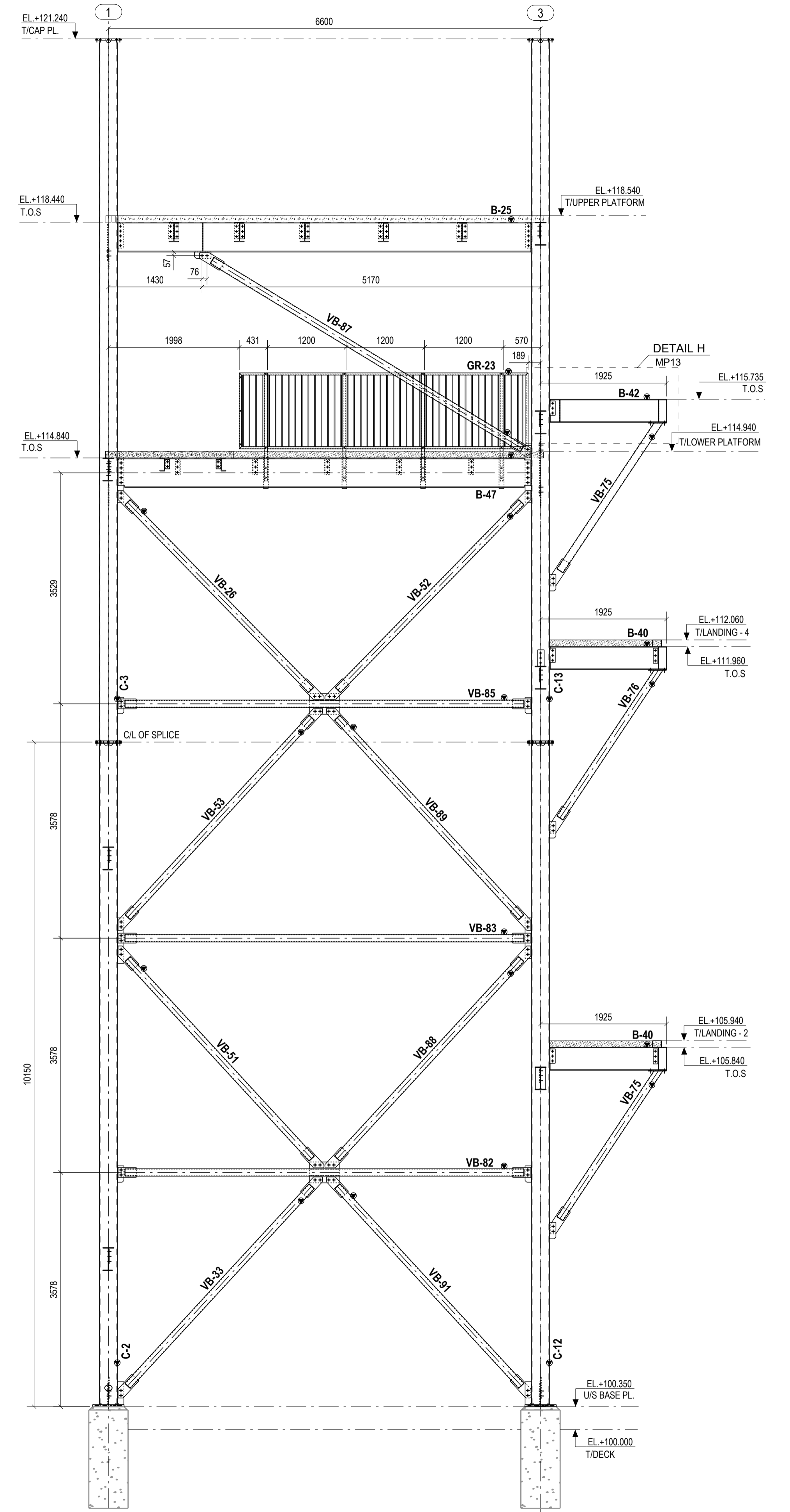
FRAME ALONG BAYLINE C
