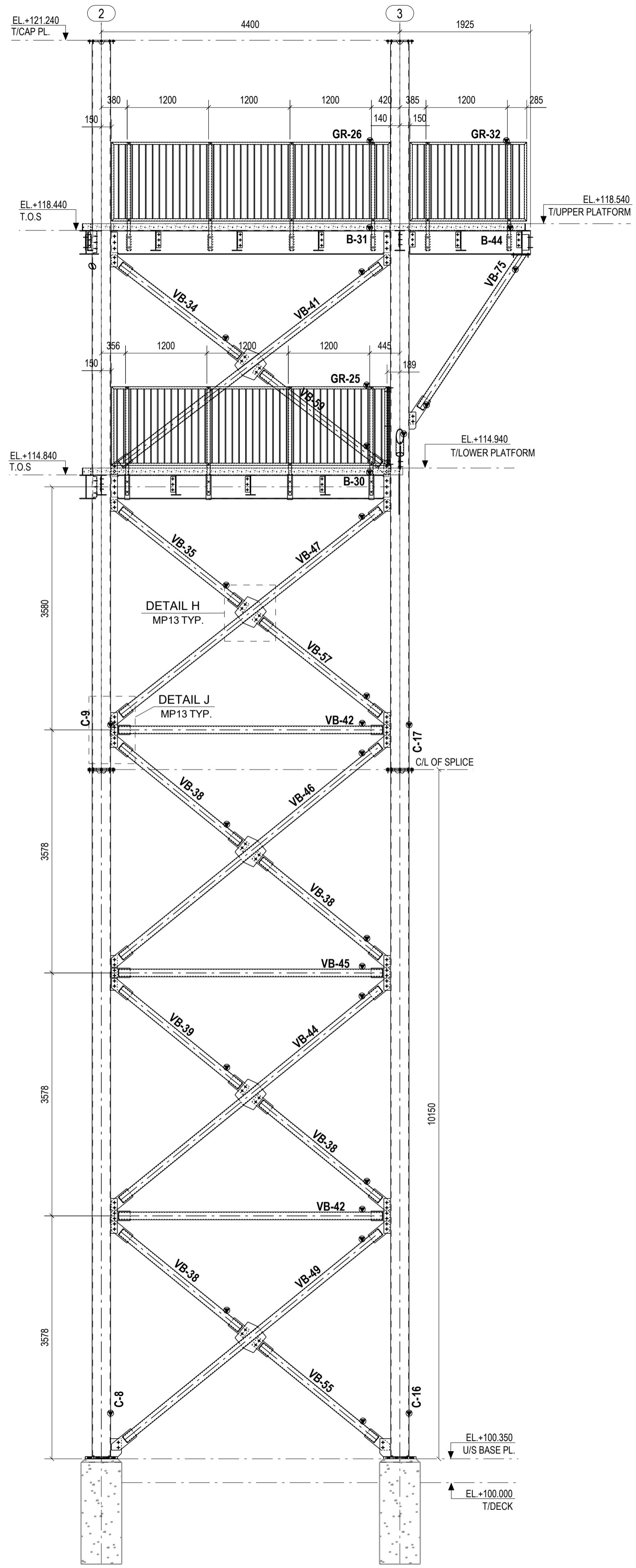
FRAME ALONG BAYLINE A
