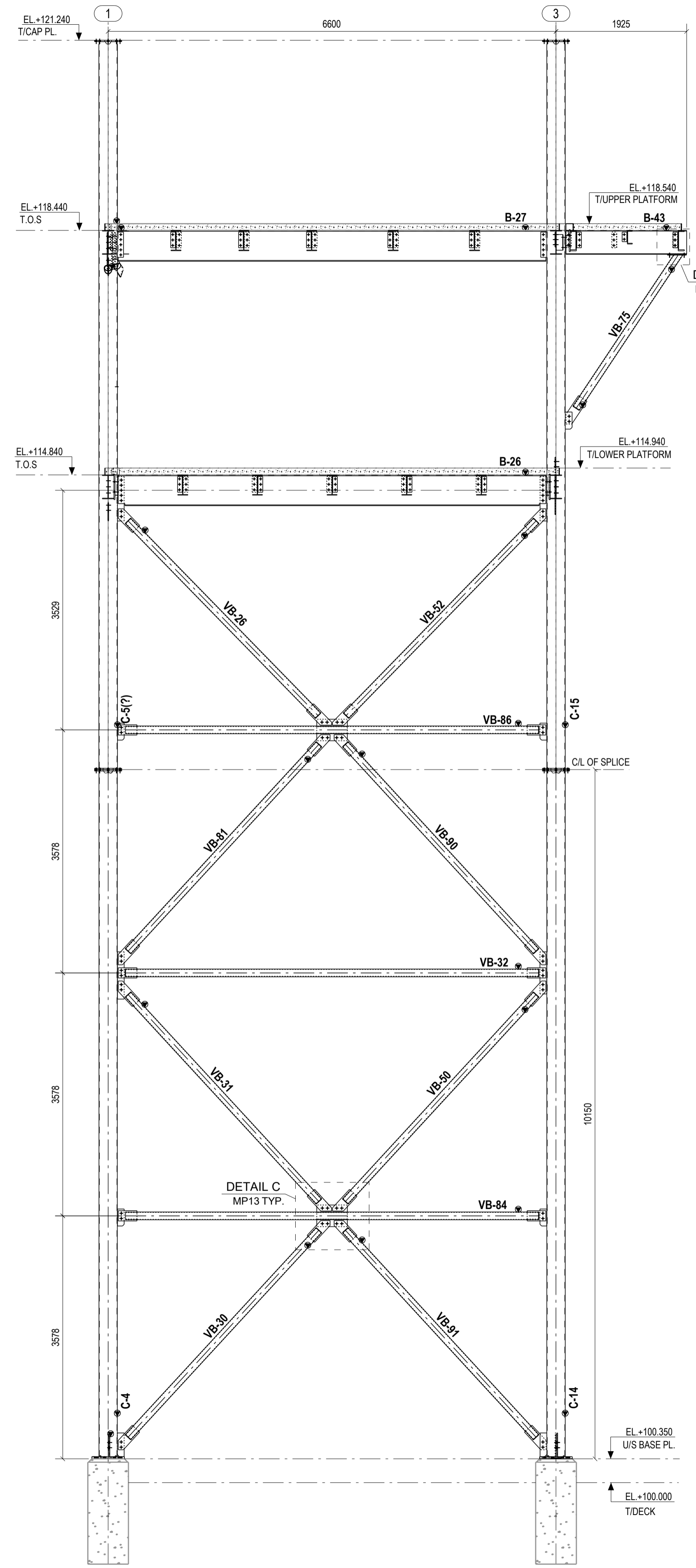
FRAME ALONG BAYLINE B
